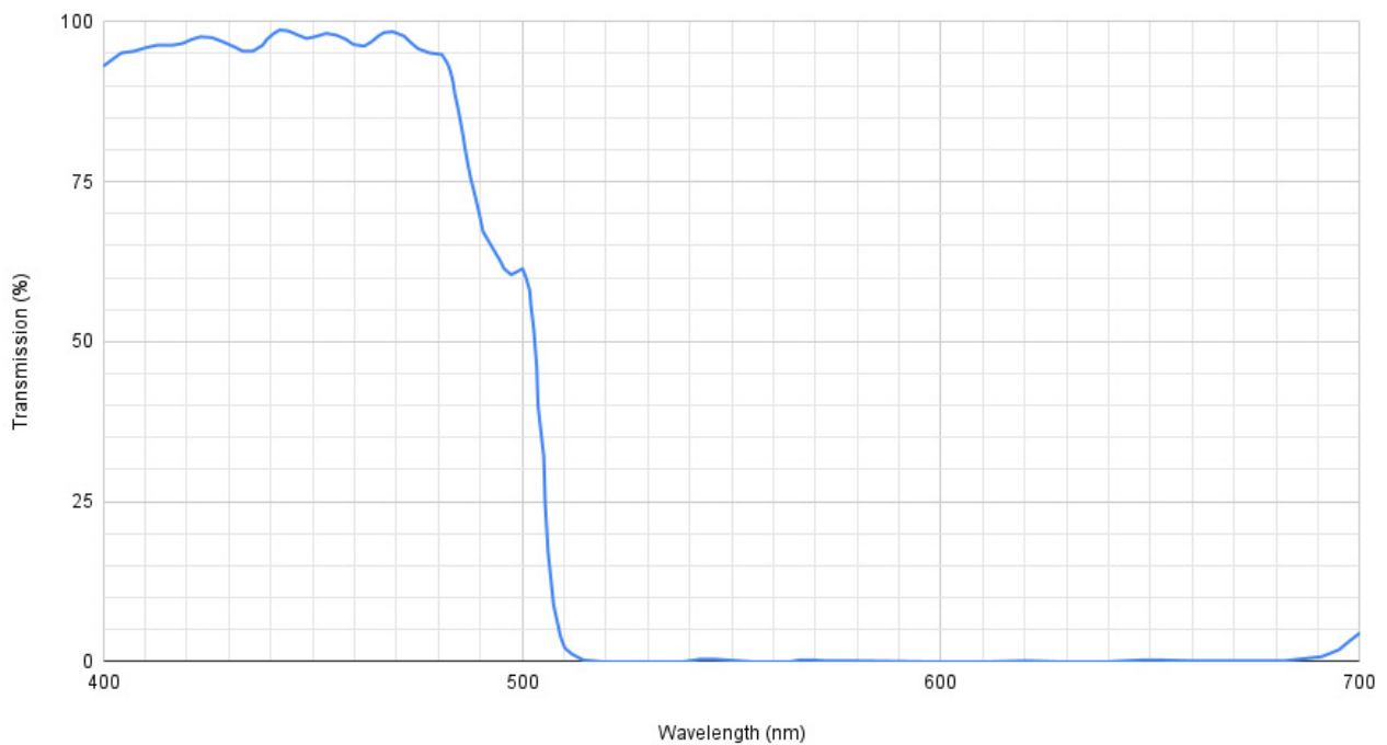
Dichroic Filter "refl. red/green"
