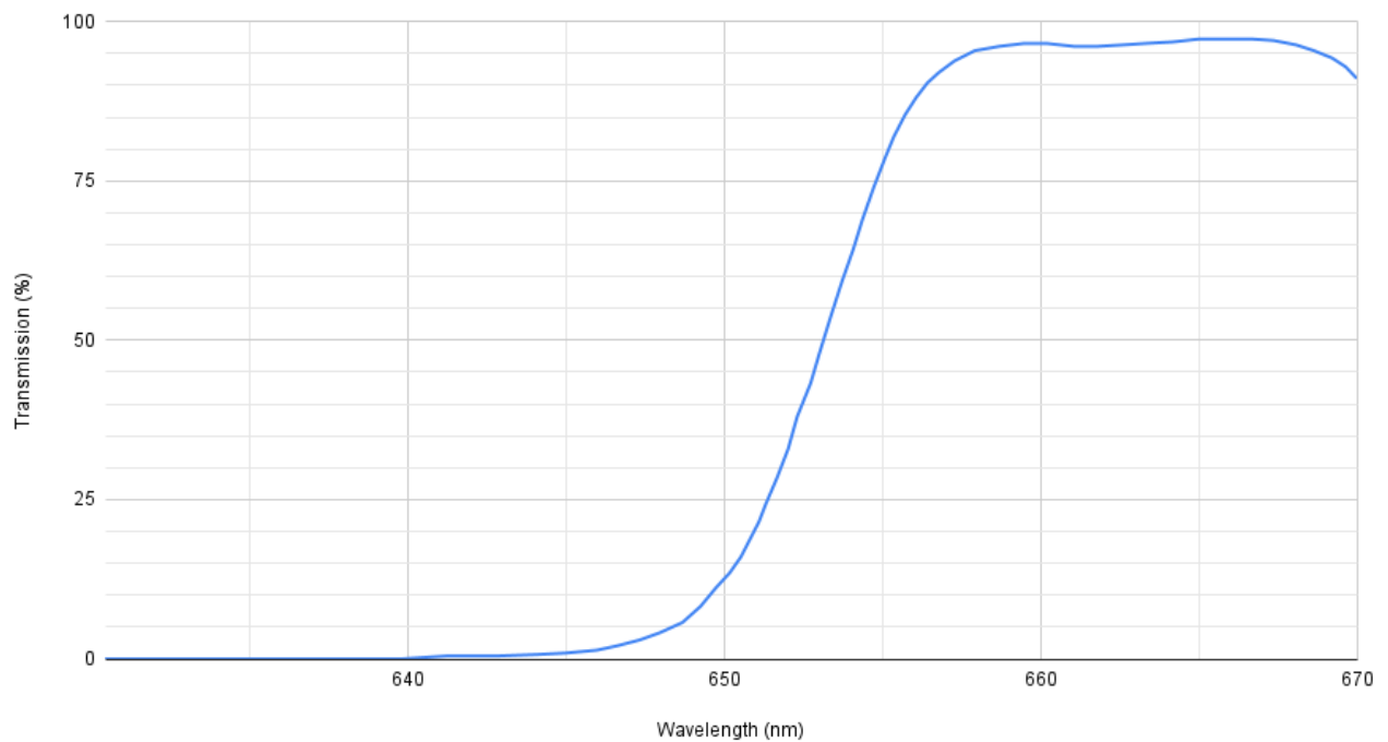
Dichroic Filter "red/red"
