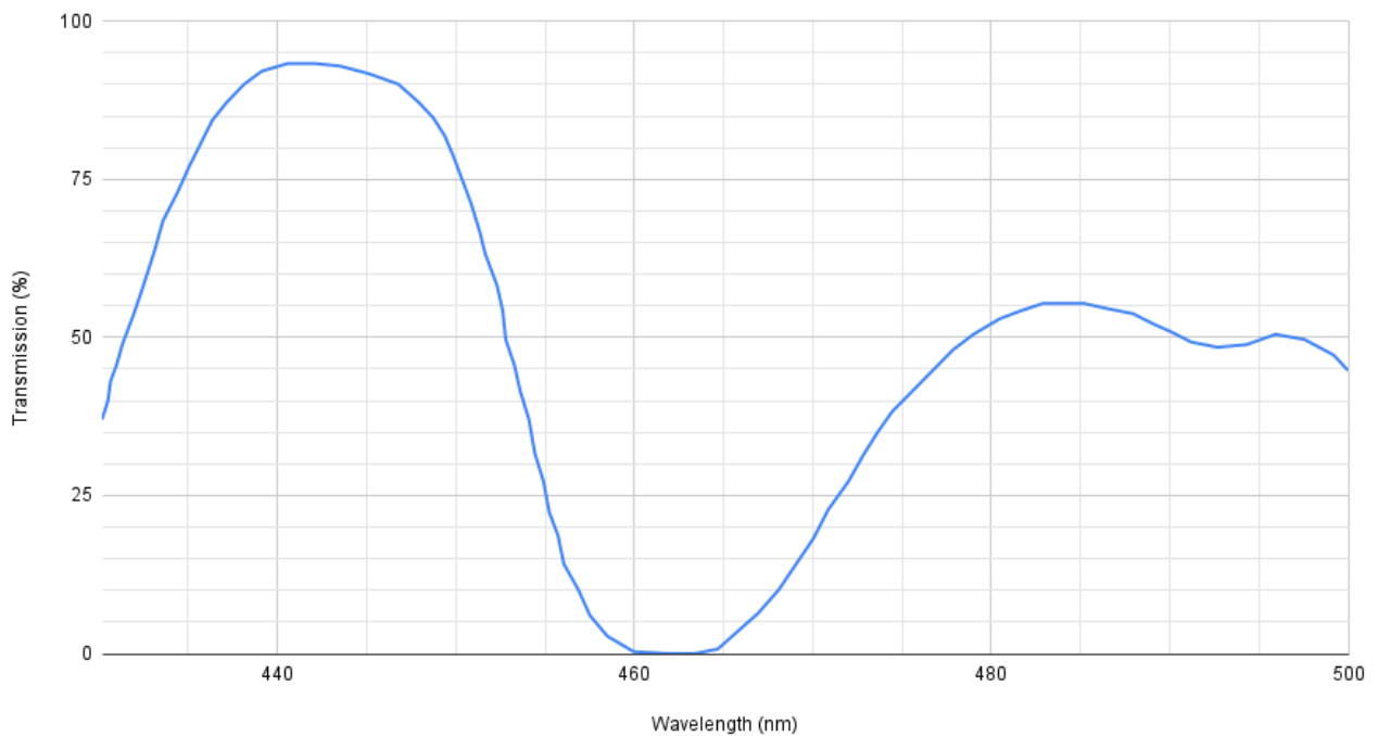
Dichroic Filter "blue/blue"
